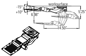
Trackless Keyboard Support Mechanism
