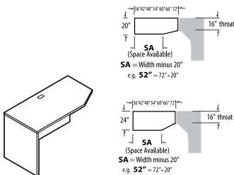
Space Saver Return - LEFT
