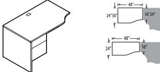
Space Saver Return - LEFT*
