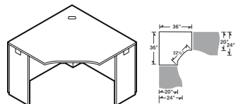
5-Sided Corner, 20" Throat
