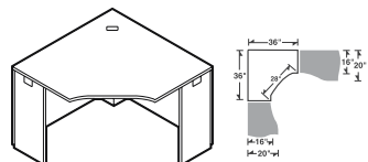
5-Sided Corner, 16" Throat
