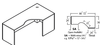
Right Extended Corner, 24" Throat Freestanding
