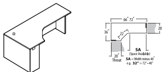
Left Extended Corner, 20" Throat
